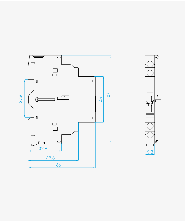
Side Mounting: Auxiliary Switch
