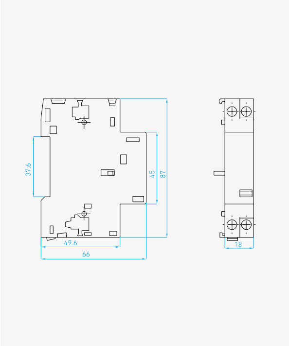
Side Mounting: Shunt Trip/UVT
