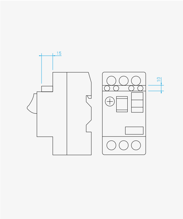
Top Mounting: Auxiliary Switch
