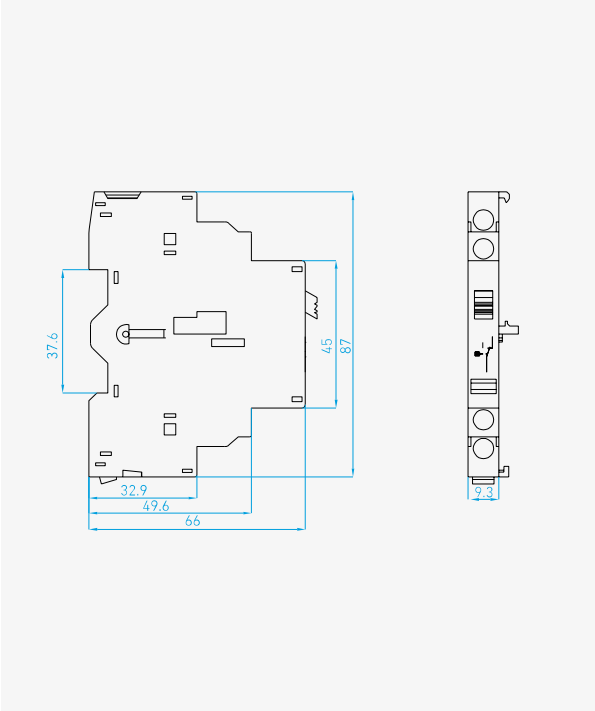
Side Mounting: Alarm Switch
