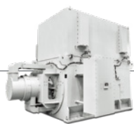
Synchronous Motor · Rated Output: < 40 MW · Rated Voltage: < 15 kV · Poles: > 2P
