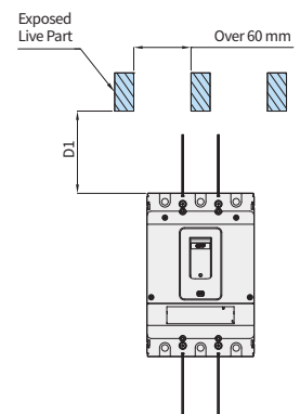
Distance with circuit breaker in case the live part is exposed
