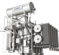
Distribution Transformer · up to 36 kV, 50 MVA
