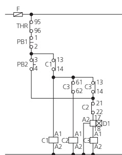
Connection Diagram 1 (HGC9 - 100)
