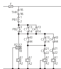
Connection Diagram 2 (HGC115 - 800)
