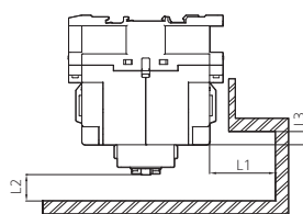
Insulation Distance
